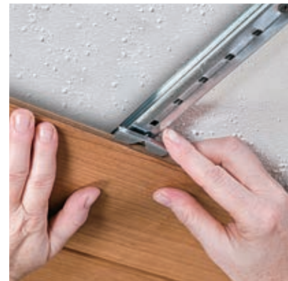
WoodHaven™ plank installation using Easy Up® tracks and clips
